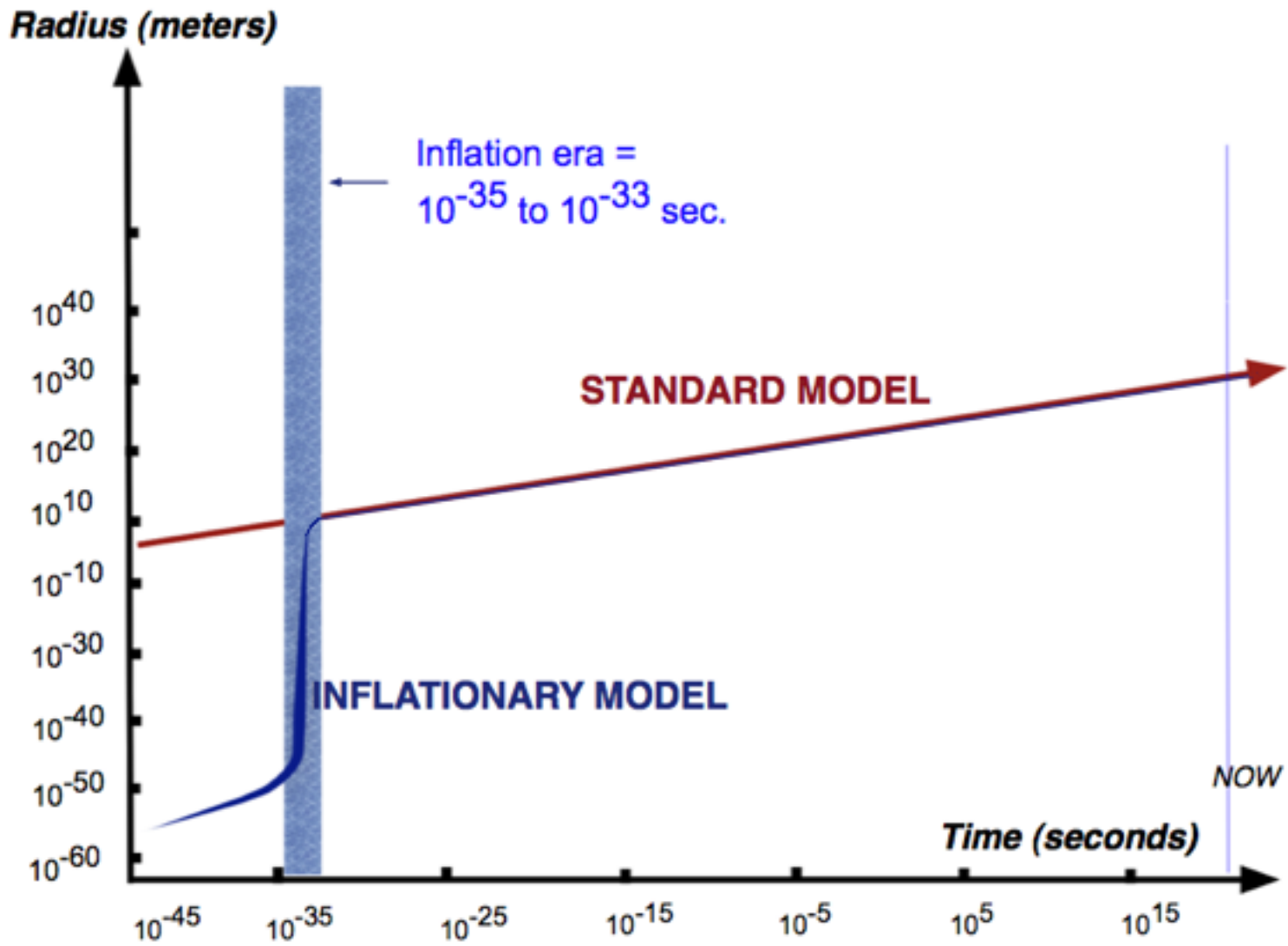
EXPANSION OF THE OBSERVABLE UNIVERSE
