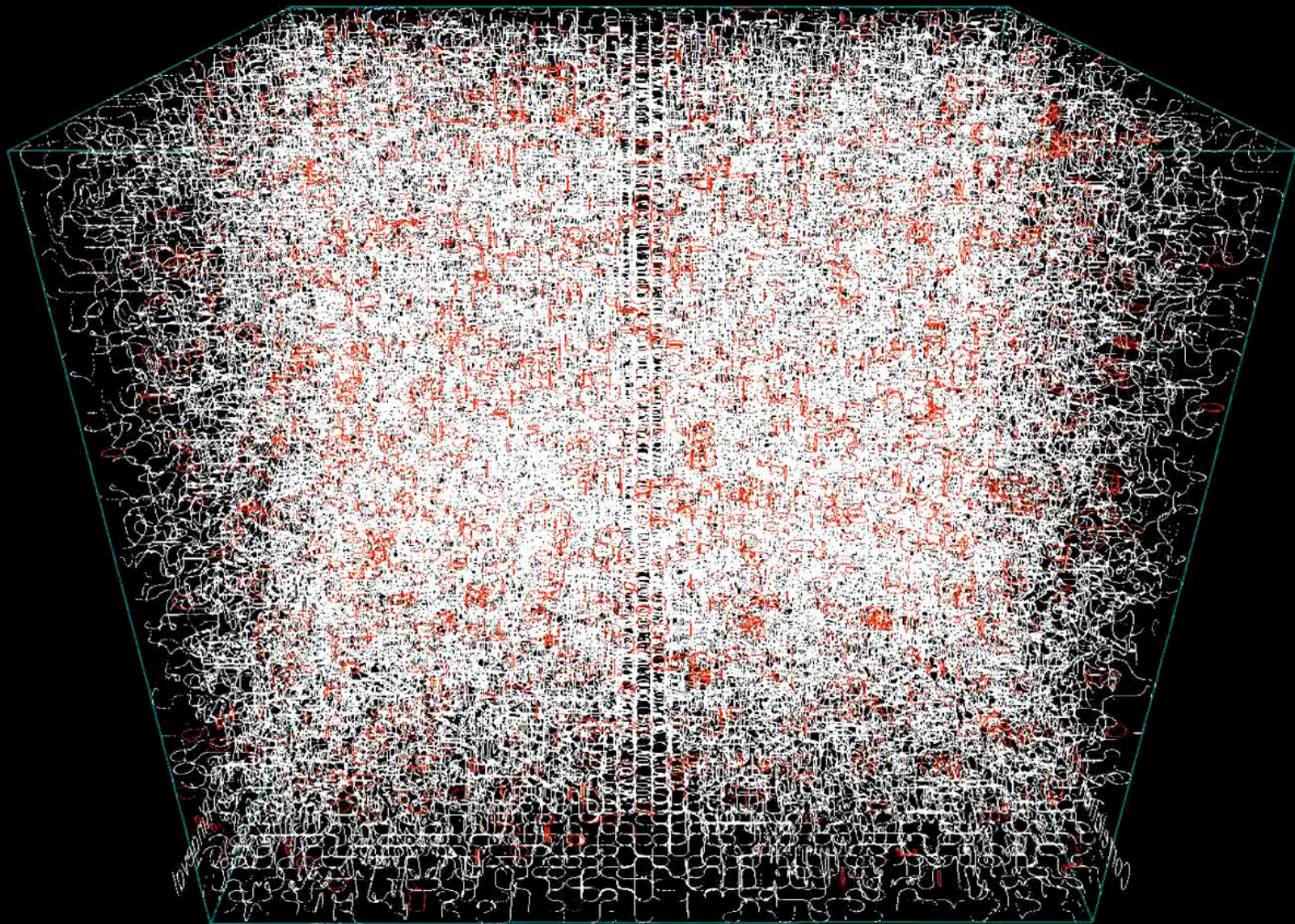
Cosmic Strings Simulation in FLRW Spacetime
