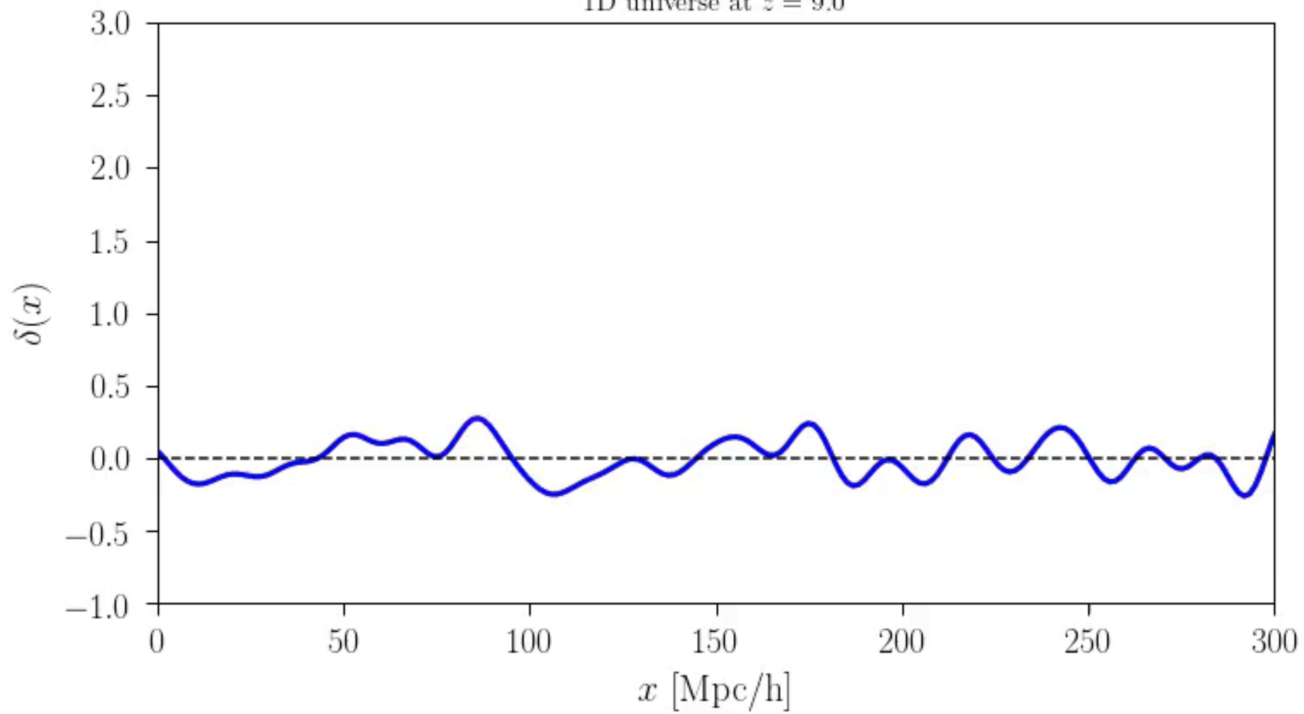
1D universe at z = 9.0
